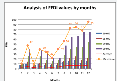
Figure 3: Comparative monthly FFDI values for Sydney Airport (showing mean, percentile and maximum values over the period 1976-2009).
