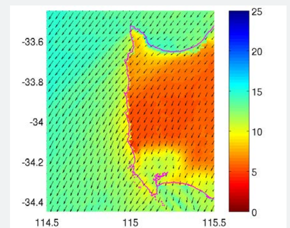
Figure 2: Surface dewpoint temperature ( ^{\circ}\text{C} ) and winds (arrows) at 8 am WST over southwest WA. Warmer colours indicate drier air.
