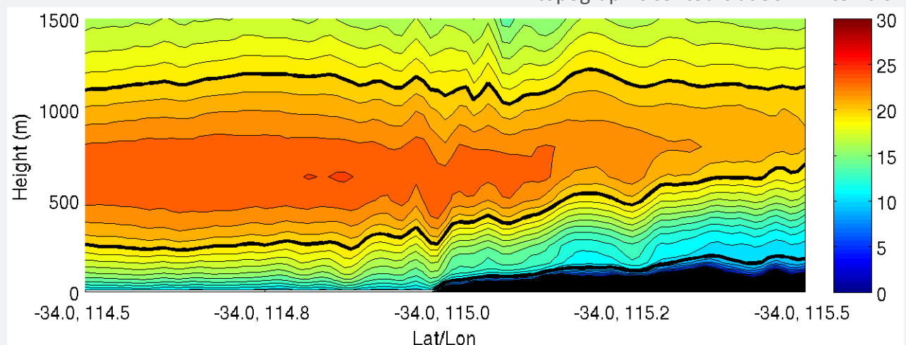
Figure 1: East-west cross-section of the wind speed at 8 am WST along latitude 34^{\circ}\text{S} . The wind speed is in \text{m s}^{-1} , contoured at 1 \text{ m s}^{-1} with multiples of 10 shown bold.
