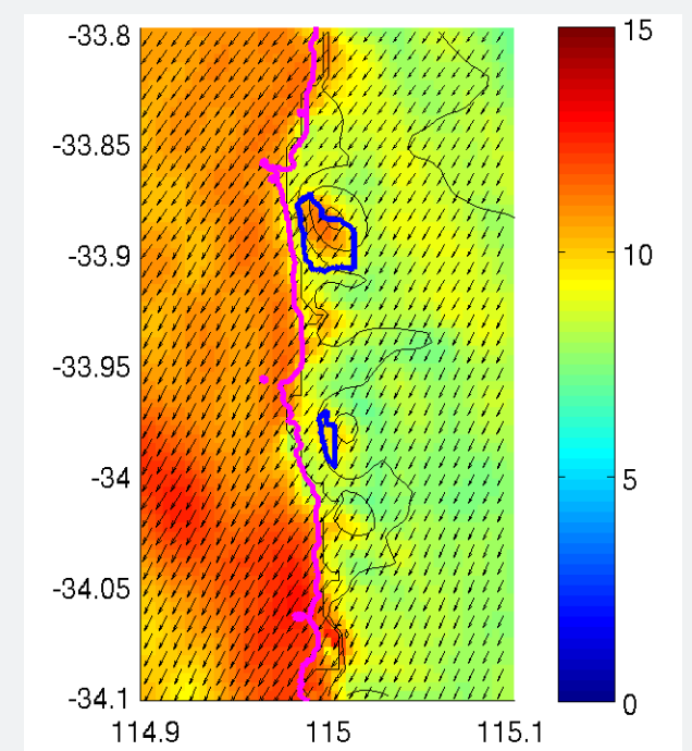
Figure 3: Surface wind speed (shading, \text{m s}^{-1} ) and vector (arrows) in the Ellensbrook – Margaret River area at 8 am WST. The blue curves show the planned burn areas and the thin black lines are topographic contours at 50-m intervals.
